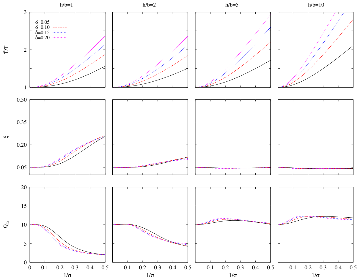
Figure 5: Effective period \tilde{T}/T , damping ratio \tilde{\xi} and maximum structural response value Q_m for a 3 \times 3 pile group with L/d = 7.5 , L/b = 1 , \xi = 0.05 , Ep/E_s = 10^3 and \xi_s = 0.05 . Influence of the mass density ratio \delta
