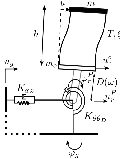
Figure 3: Equivalent model with diagonalized impedance matrix
