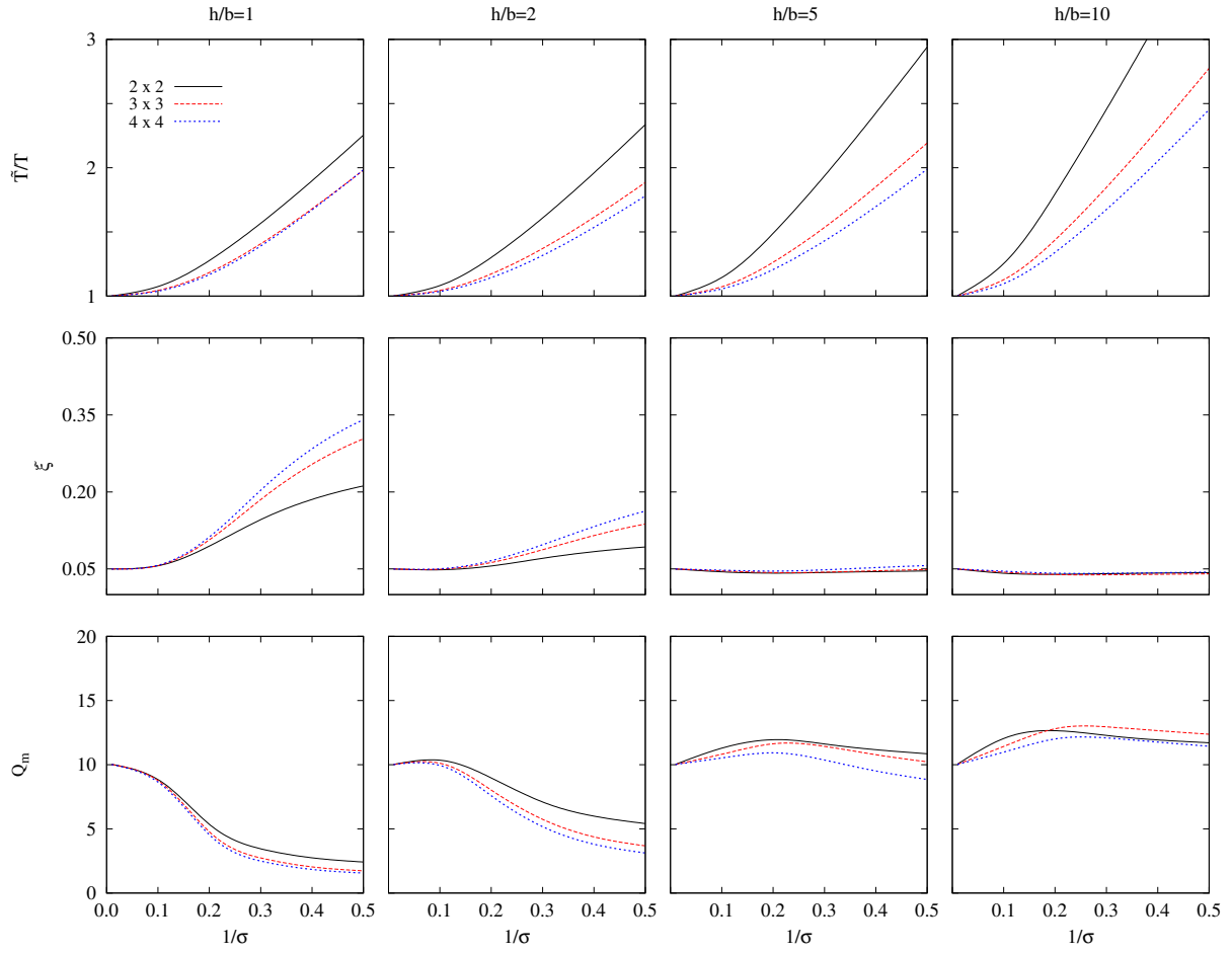
Figure 10: Effective period \tilde{T}/T , damping ratio \xi and maximum structural response value Q_m for pile groups with L/d = 15 , L/b = 2 and \xi_s = 0.05 . Influence of pile group size
